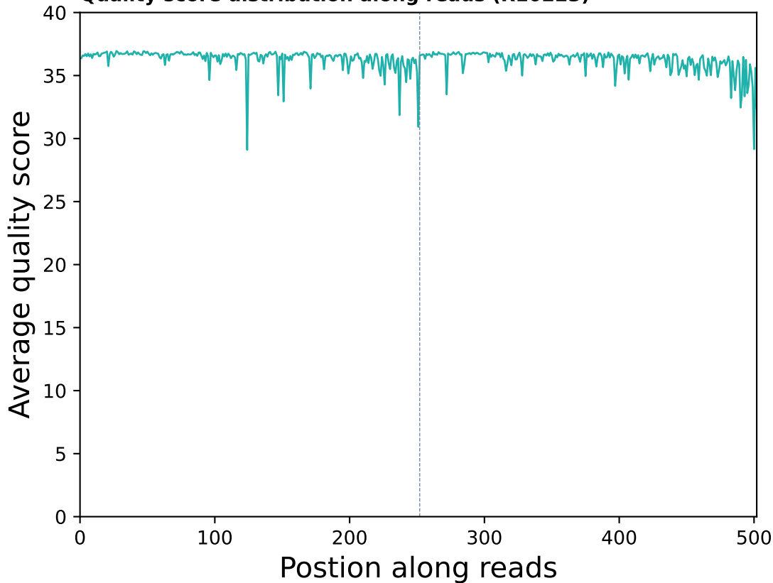
Quality score distribution along reads (R10223)
